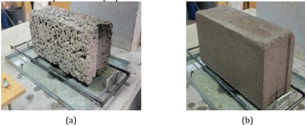
Fig. 9. Specimens selected for visual inspection, dimension measurement, and absorption testing (a) Caramelo block and (b) Pressed block
