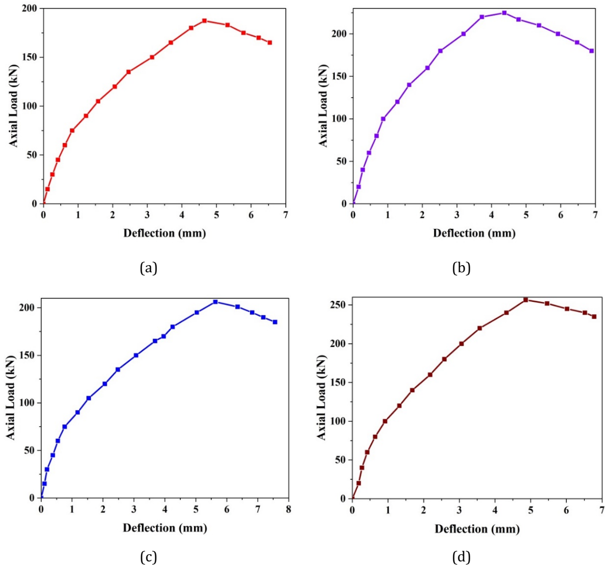
Fig. 19. Axial load-deflection response from an experimental study (a) M40-SF0.8-B0-S100, (b) M40-SF0.8-B0-S80, (c) M40-SF0.8-B2-S100, and (d) M40-SF0.8-B2-S80
