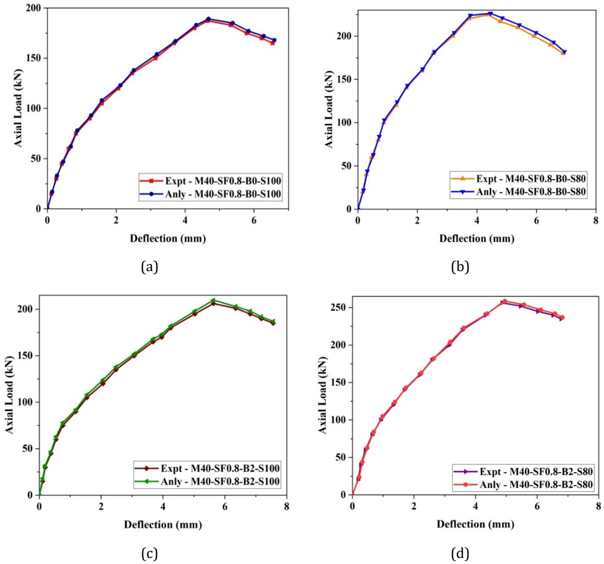
Fig. 21. Comparison of the experimental and analytical axial load-deflection response of all RC beams (a) M40-SF0.8-B0-S100, (b) M40-SF0.8-B0-S80, (c) M40-SF0.8-B2-S100, and (d) M40-SF0.8-B2-S80
