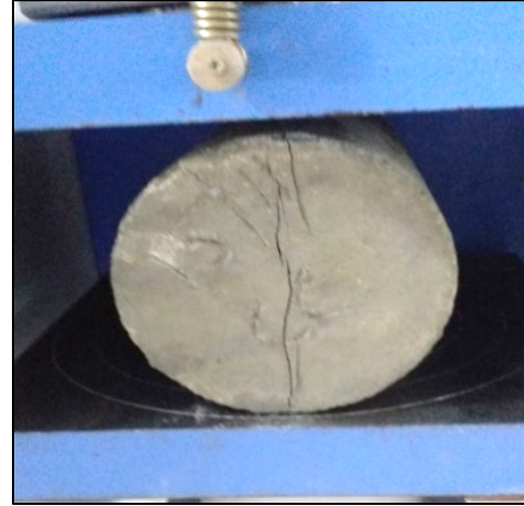
Fig. 5. Split tensile strength test
