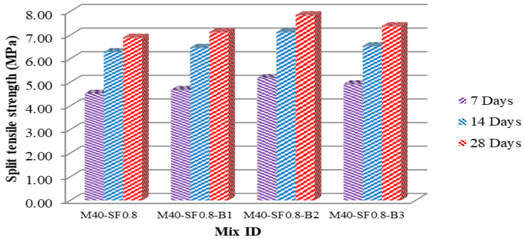
Fig. 16. STS of steel fibre concrete with microorganisms at various ages
