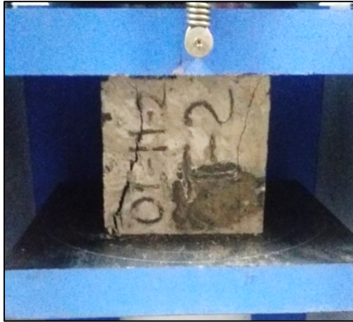
Fig. 4. Compressive strength test
