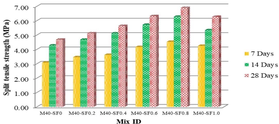
Fig. 15. Split tensile strength of steel fibre concrete at various ages
