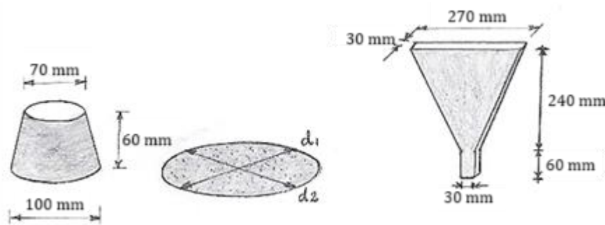
Fig. 3. Mini slump and V-funnel testing equipment
