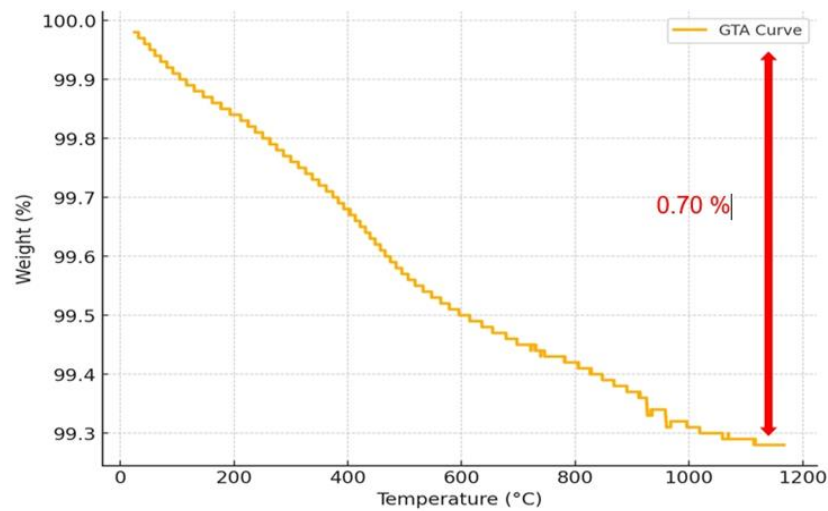
Fig. 12. Gravimetric Thermal Analysis (GTA) curve of dune sand and crushed dune sand
