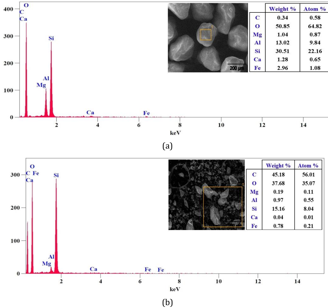
Fig. 5. SEM-EDS test results of (a) Dune sand and (b) Crushed Dune Sand
