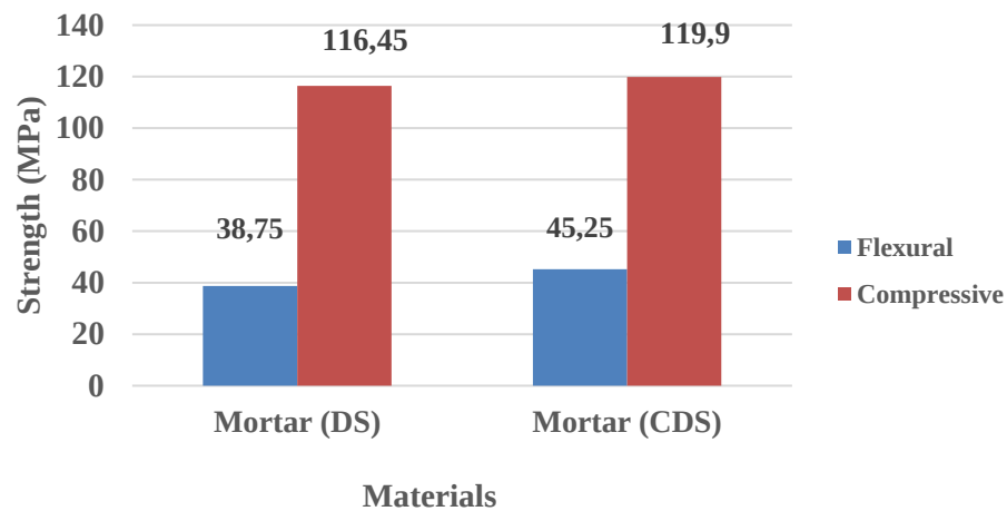
Fig. 8. Strength of treated leveling mortar
