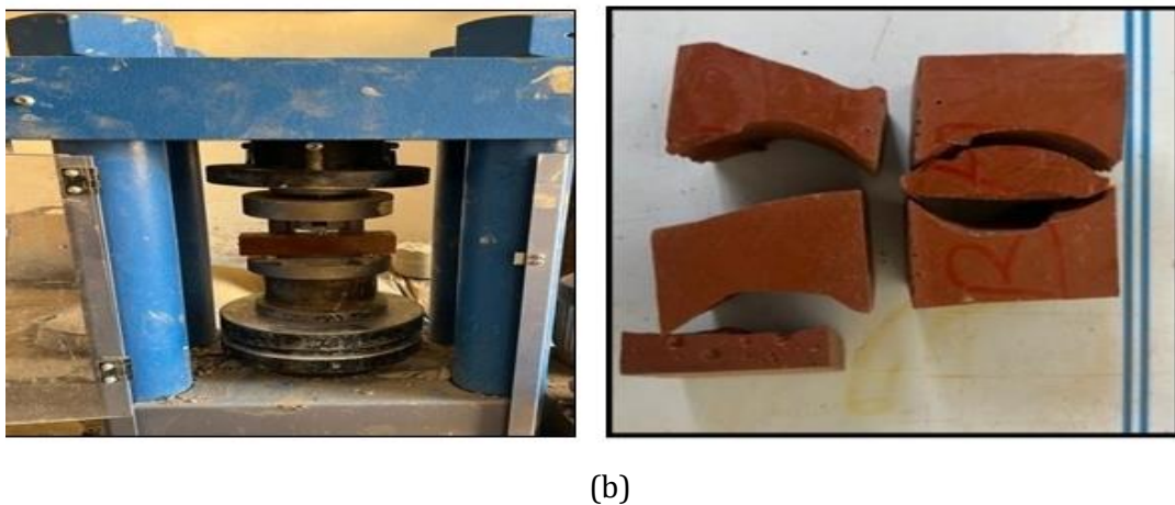
Fig. 3. Mechanical test (a) compression and (b) flexural of leveling mortars
