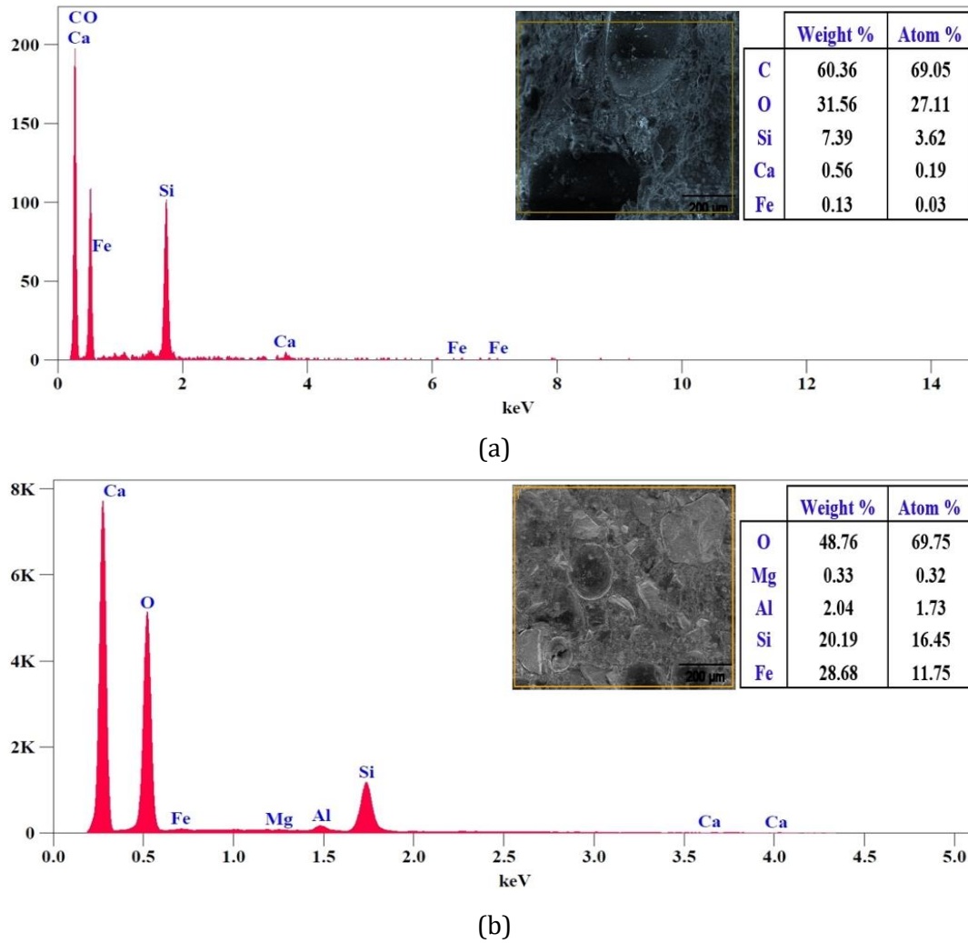
Fig. 6. SEM-EDS test results of (a) Leveling mortar (M) and (b) Treated Leveling mortar (TM)
