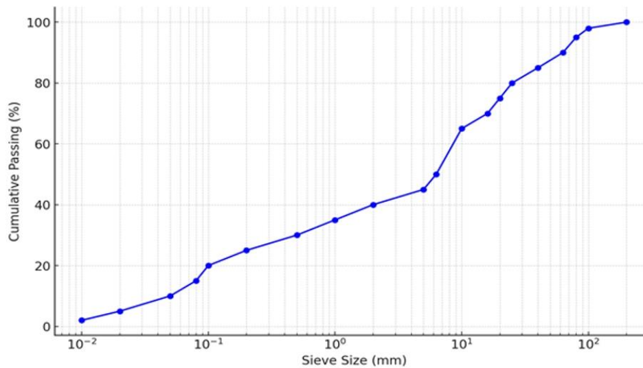
Fig. 1. Particle size distribution curve of Crushed dune sand
