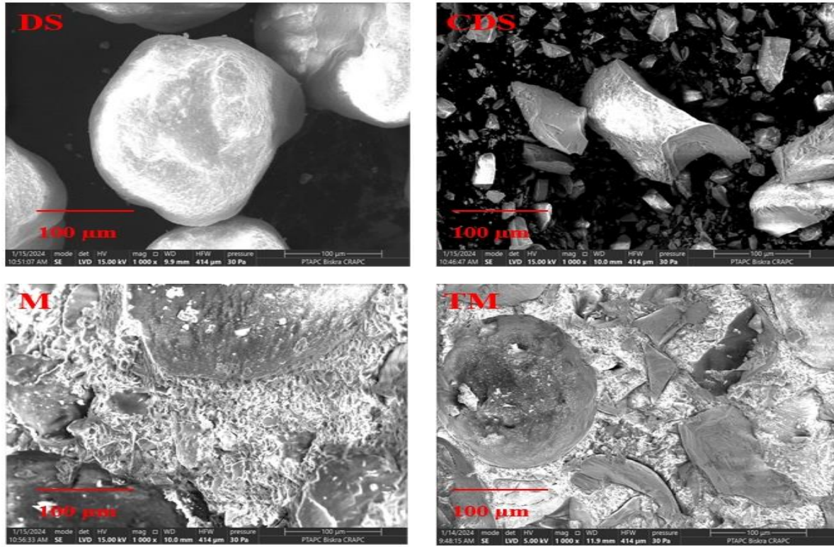
Fig. 4. SEM micrographs of dune sand (DS), Crushed Dune Sand (CDS), leveling mortar (M), treated leveling mortar (TM)
