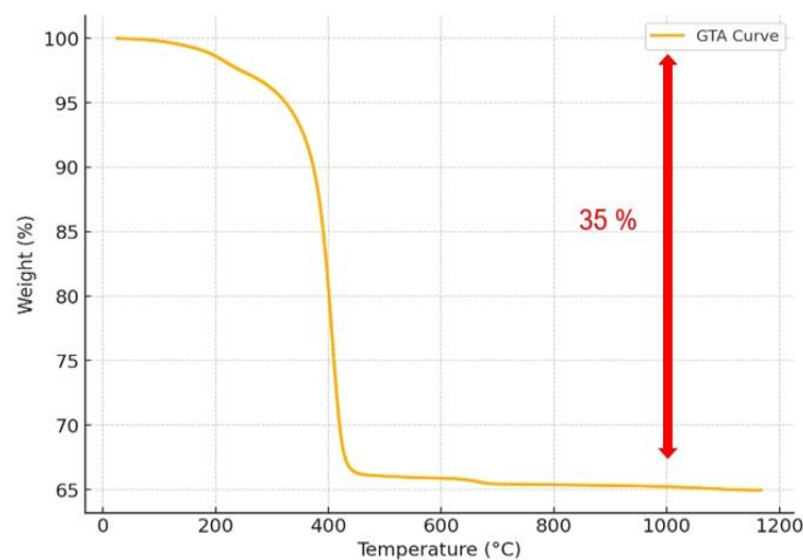
Fig. 13. Gravimetric Thermal Analysis (GTA) curve of leveling mortar and treated leveling mortar
