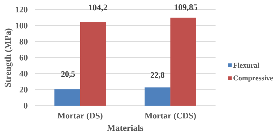
Fig. 7. Strength of leveling mortar without heat treatment
