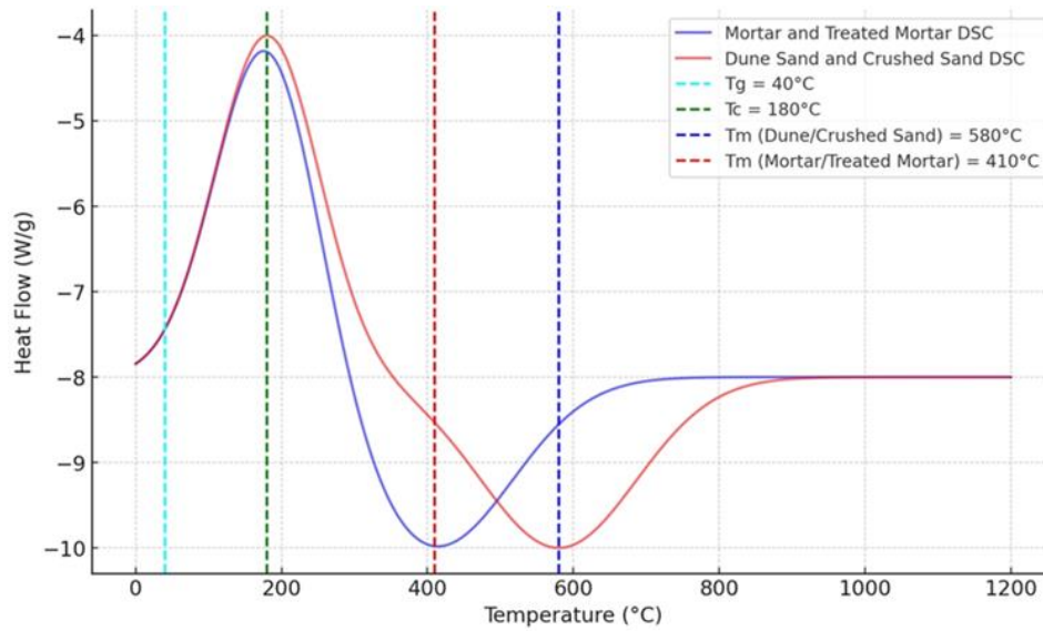
Fig. 9. Differential scanning calorimetry (DSC) curve of dune sand, crushed dune sand, leveling mortar and treated leveling mortar
