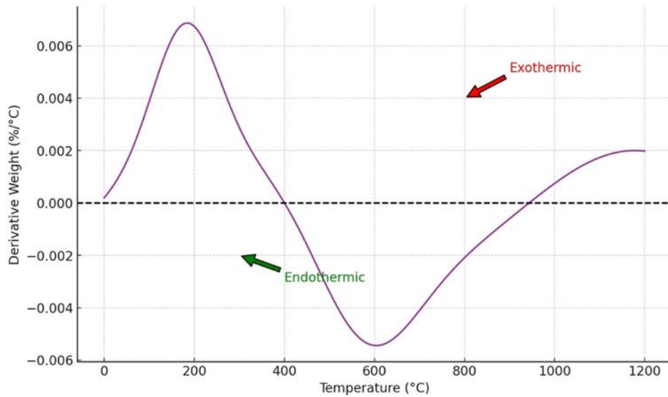
Fig. 10. Differential Thermal Analysis (DTA) curve of dune sand and crushed dune sand
