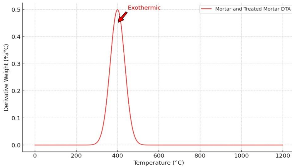
Fig. 11. Differential Thermal Analysis (DTA) curve of leveling mortar and treated leveling mortar
