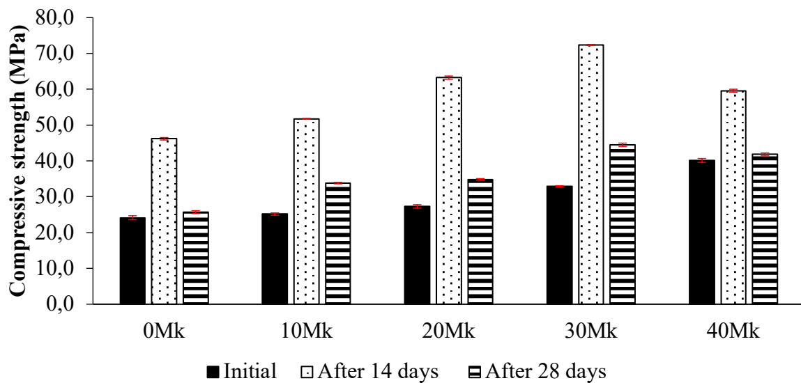
Fig. 10. Compressive strength findings of geopolymer samples with differing metakaolin proportions prior to and following 14 and 28 days of exposure to sulfuric acid
