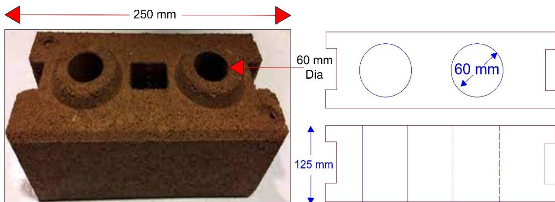
Fig. 1. Brick geometry
