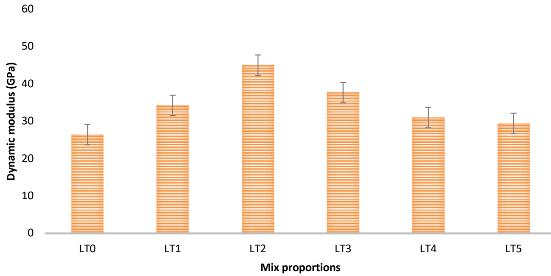
Fig. 8. Variation of the dynamic modulus of LTC
