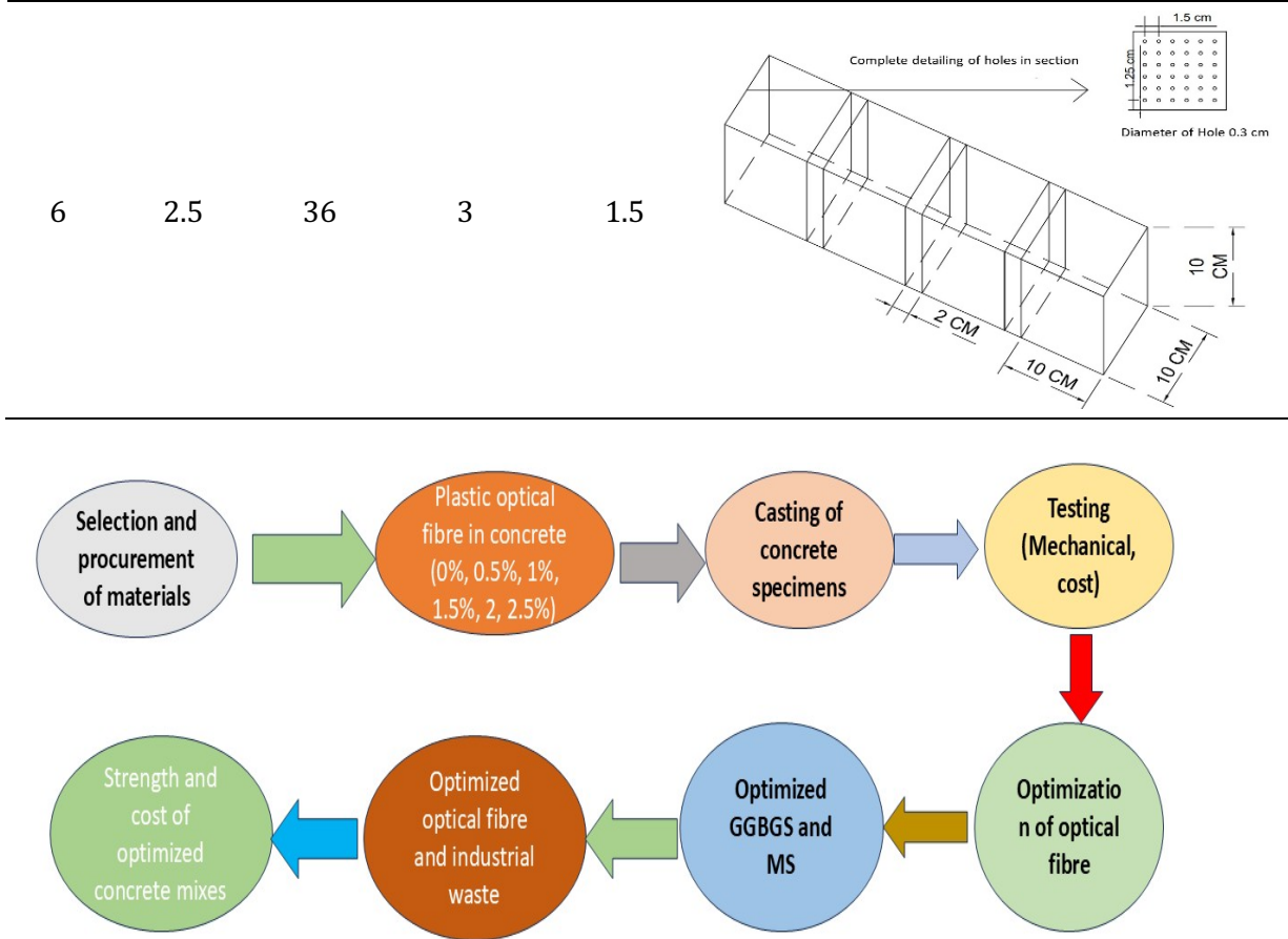
Fig. 2. Methodology for the experimental program of LTC
