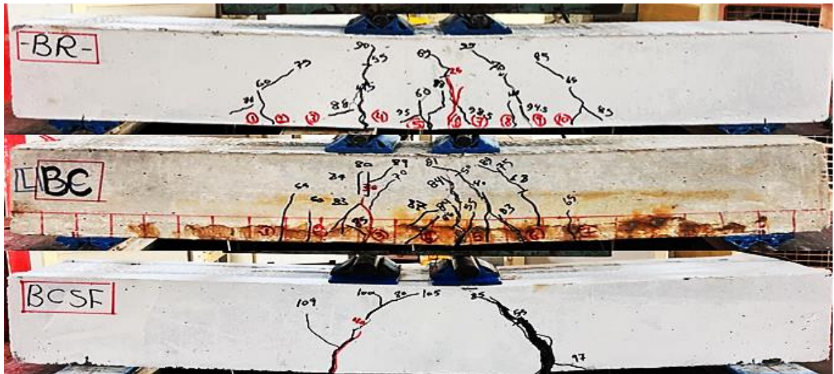
Fig. 9. Failure modes
