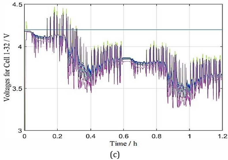
Fig. 24. Test case 5: Overvoltage during regenerative braking (a) Pack voltage and pack current in time (b) Switch box contactor logic and (c) Cell voltages in time and max. voltage threshold [95]
