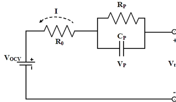
Fig. 12. Equivalent circuit of the battery
