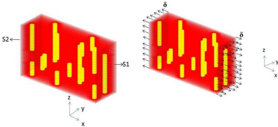
Fig. 7. The displacement \delta applied to the RVE
