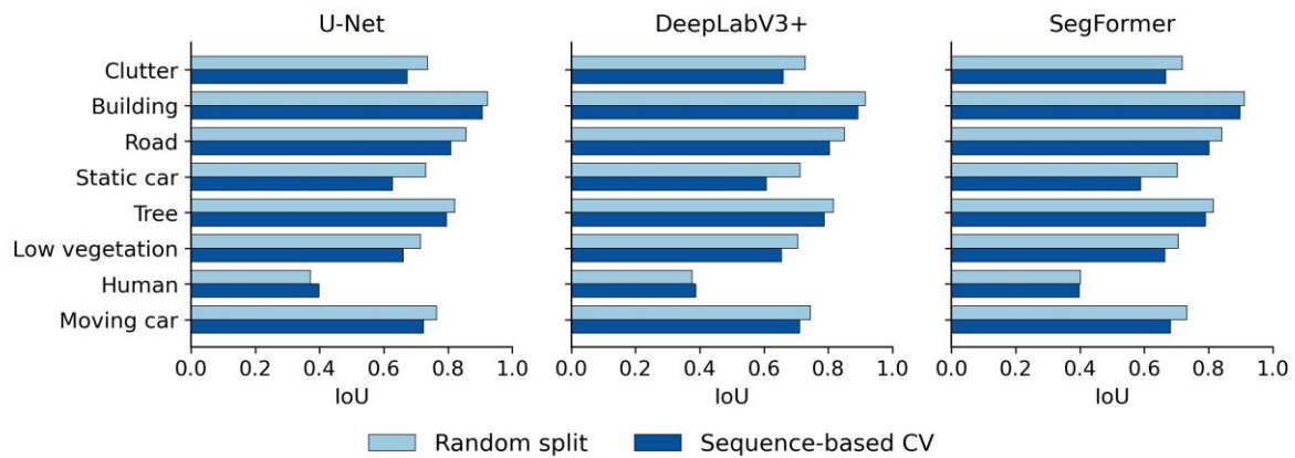
Fig. 6. Class-wise IoU of the three models under the random split and the sequence-based spatial cross validation
