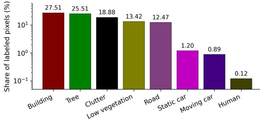
Fig. 4. Share of labeled pixels per class (logarithmic scale)
