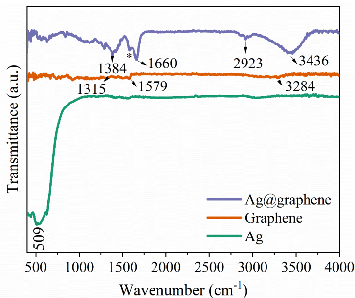
Fig. 2. FTIR spectra of AgNPs, graphene, and Ag@graphene nanocomposite in the wavelength ranging from 400 to 4000 \text{cm}^{-1}
