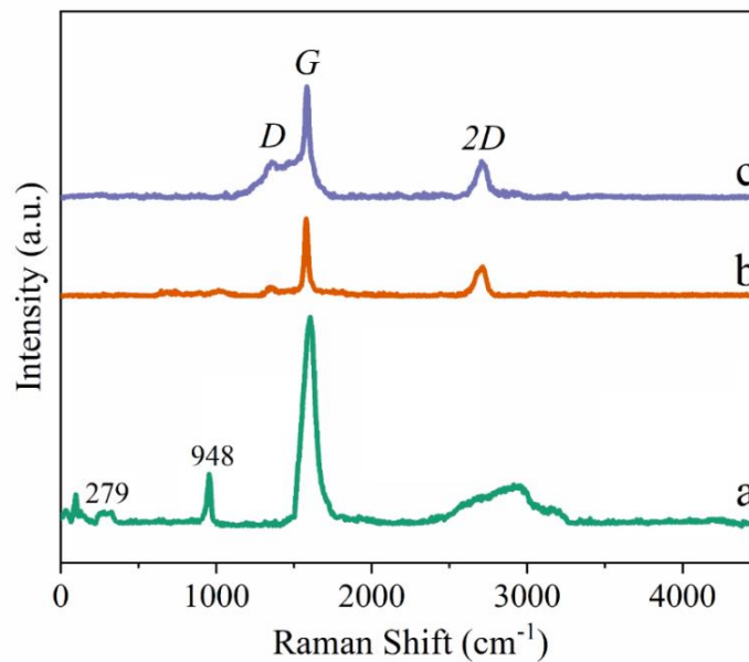
Fig. 6. Raman spectra of (a) AgNPs, (b) graphene, and (c) Ag@graphene nanocomposite
