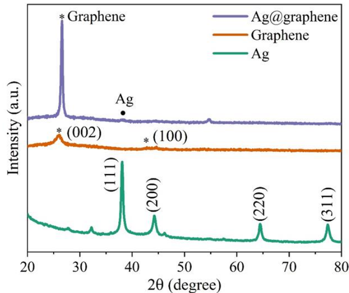
Fig. 1. XRD patterns of AgNPs, graphene, and Ag@graphene nanocomposite
