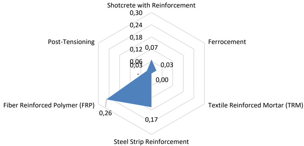
Fig. 3. Diagram of strengthening technique's performance
