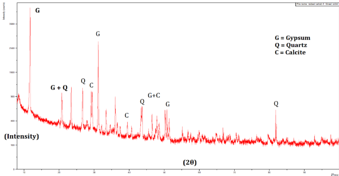
Fig. 15. XRD pattern for untreated gypseous soil
