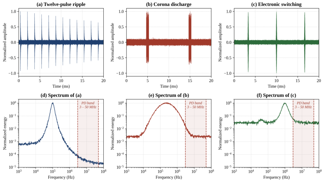
Fig. 2. Comparison of time-frequency characteristics of three typical pulse-type interference signals
