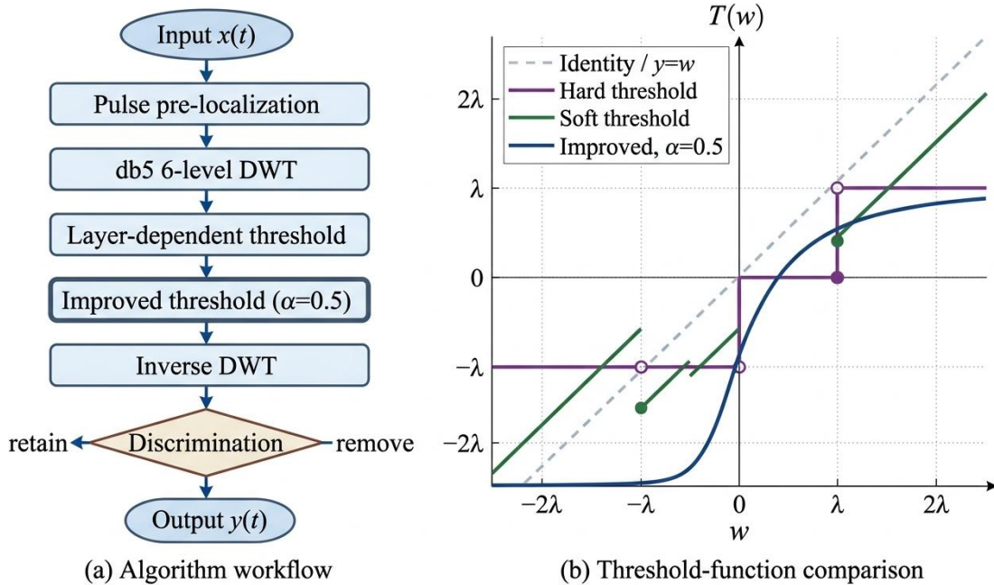
Fig. 3. Overall workflow of the improved wavelet threshold algorithm together with a comparison of the core threshold functions: (a) algorithm workflow; (b) comparison of the proposed continuously differentiable threshold function ( \alpha = 0.5 ) with the hard and soft threshold functions
