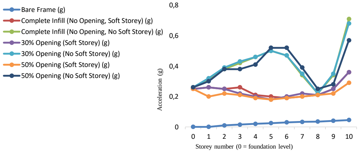
Fig. 12. Story acceleration under soft rock conditions
